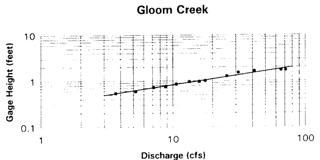
Figure 55. Rating curve for Gloom Creek, Bighorn National Forest.
