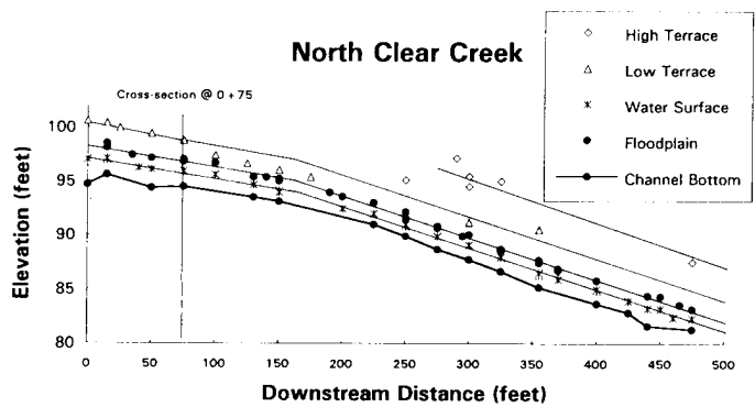
Figure 53. Office plot of longitudinal profile survey.
