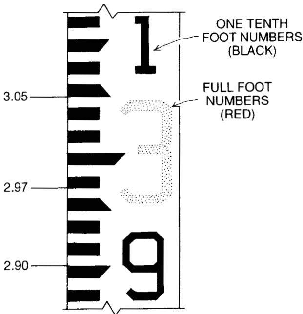
Figure 22. Leveling rod.
