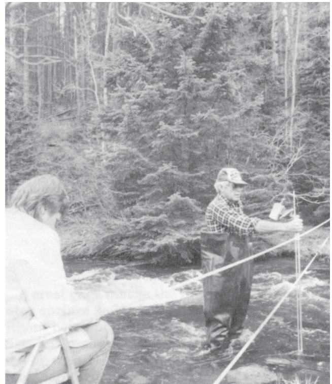
Figure 57. Measuring current velocity with a Price AA flow meter.
